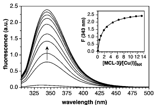
Figure 7. Fluorescence titration of CusF (20 \mu M) with MCL-3 at pH 7.0 (50 mM MOPS, 0.15 M NaCl, 25 ^{\circ} C). Inset: Change of the fluorescence intensity at 343 nm (excitation at 290 nm).
