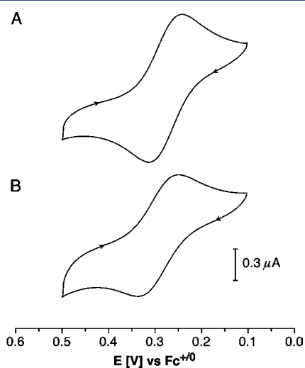
Figure 4. Cyclic voltammograms for (A) MCL-1 (150 \mu\text{M} ) and (B) MCL-3 (150 \mu\text{M} ) in the presence of \text{CuSO}_4 (1 mM) at pH 5.0 (10 mM PIPBS, 0.1 M \text{KClO}_4 ; glassy carbon electrode, scan rate 20 mV/s).
