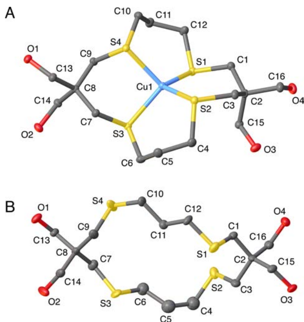
Figure 2. ORTEP drawings and atom numbering schemes for the crystal structures of (A) [Cu(I)–( tr MCL-3)]PF 6 [ 16 ( 1 )] and (B) the free ligand tr MCL-3 ( 12 ). Ellipsoids shown represent 50% probability. Hydrogen atoms have been omitted for clarity.
