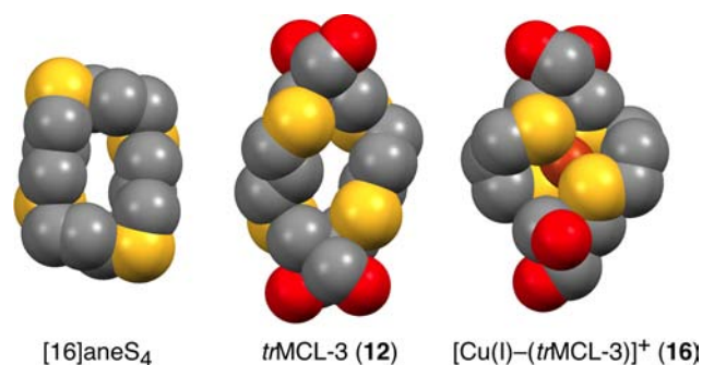
Figure 3. Space-filling models illustrating the molecular preorganization of tr MCL-3 ( 12 ) vs [16]aneS 4 34 in comparison to the geometry of [Cu(I)–( tr MCL-3)]PF 6 ( 16 ) (representations were generated with Mercury CSD 35 from crystal structure atomic coordinates).
