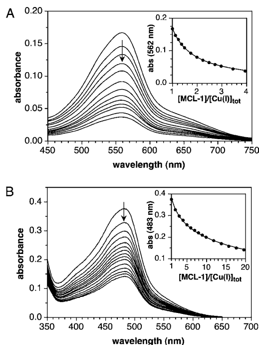
Figure 5. Spectrophotometric titrations of (A) 2,2'-bicinchoninic acid (BCA, 6 ; 100 \mu\text{M} ) at pH 5.0 (10 mM PIPBS, 0.1 M \text{KClO}_4 ) and (B) bathocuproine disulfonate (BCS, 5 ; 50 \mu\text{M} ) at pH 7.0 (10 mM PIPES, 0.1 M \text{KClO}_4 ) with MCL-1 in the presence of Cu(I).
