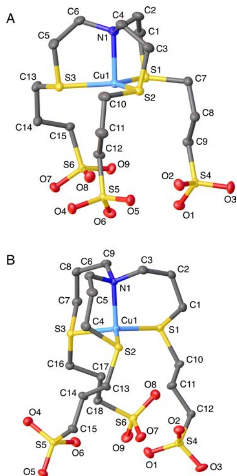
Figure 1. ORTEP drawings and atom numbering schemes for the crystal structures of the Cu(I) complexes of (A) MCL-1 ( 13a ) and (B) MCL-2 [ 14a (I) ]. Ellipsoids shown represent 50% probability. Hydrogen atoms and counterions have been omitted for clarity. A packing diagram for each structure is provided in Figure S1 in the Supporting Information.
