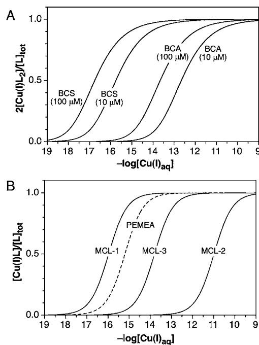
Figure 6. Dynamic range for buffering of free \text{Cu(I)}_{\text{aq}} with ligands exhibiting (A) 2:1 and (B) 1:1 complex stoichiometries. The fractional saturation of the corresponding ligand was calculated as a function of -\log [\text{Cu(I)}_{\text{aq}}] for a buffer with constant total ligand concentration and varying [\text{Cu(I)}]_{\text{total}} at pH 7.0 ( I = 0.1 ).
